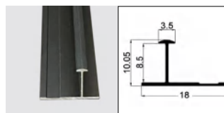
LT-A3 I-shaped line
