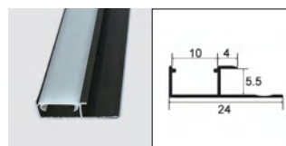
518 Side light strip
