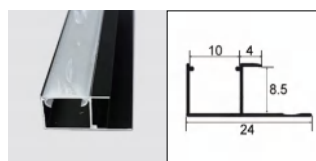
818 Side light strip
